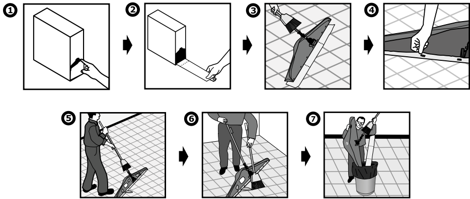
Single mold constructed dust mop head and recovery pan
